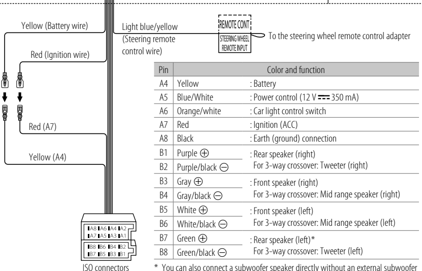
ISO connectors
